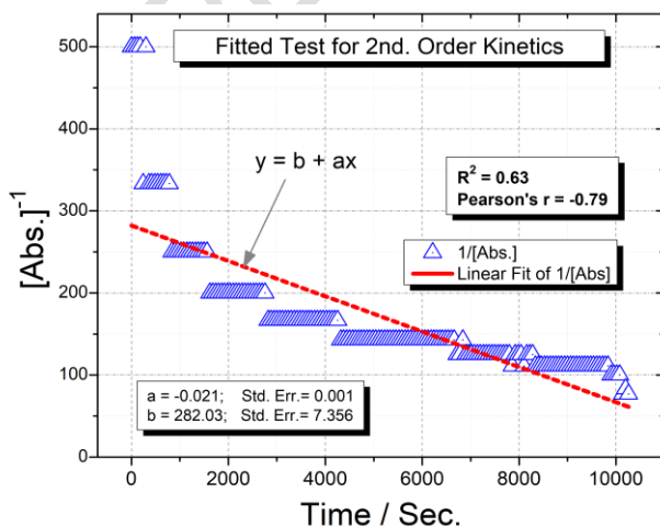
Figure 8(b): Fitted Test for Second - Order Kinetics
