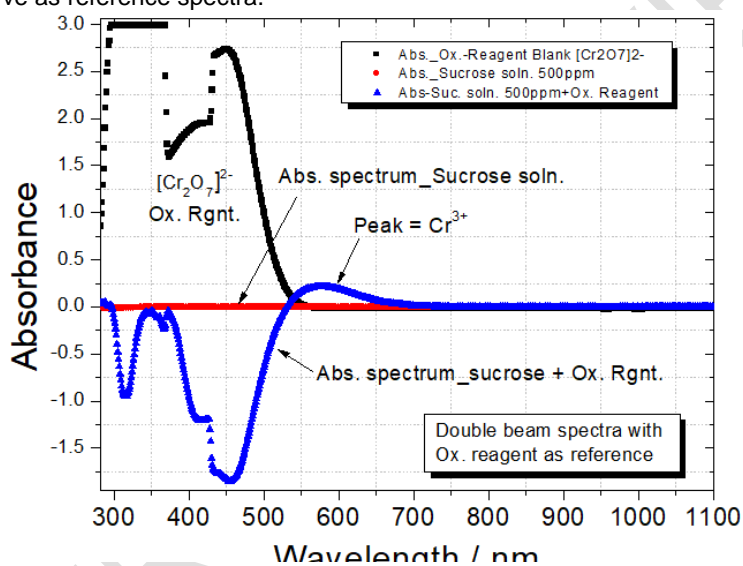
Figure 1: Electronic Absorption Spectrum of Oxidizing Reagent (reference blank), Sucrose Solution (reference blank) and Sucrose Solution (Treated with the Oxidizing Agent)
