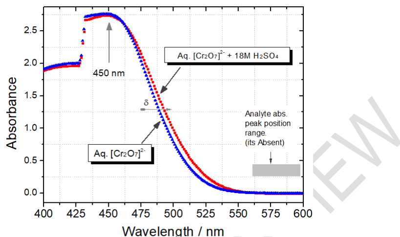
Figure 6: Broadening of the dichromate ion absorption band due to addition of 18M H 2 SO 4 acid
