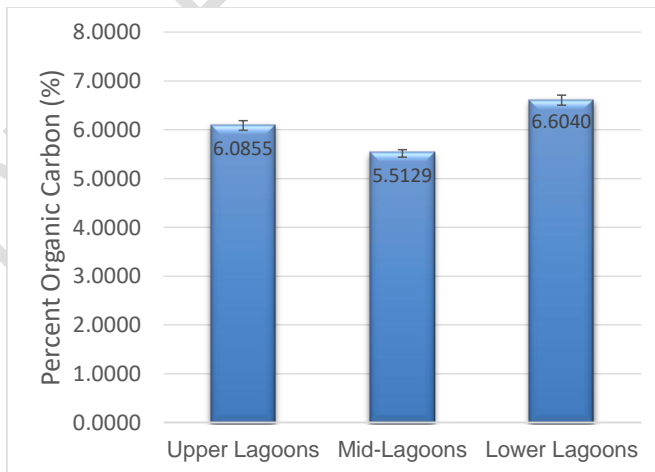
Figure13: Histogram chart comparing the percent OC obtained from upper, mid-, and lower sewage treatment plant lagoons near the banks of River Njoro
