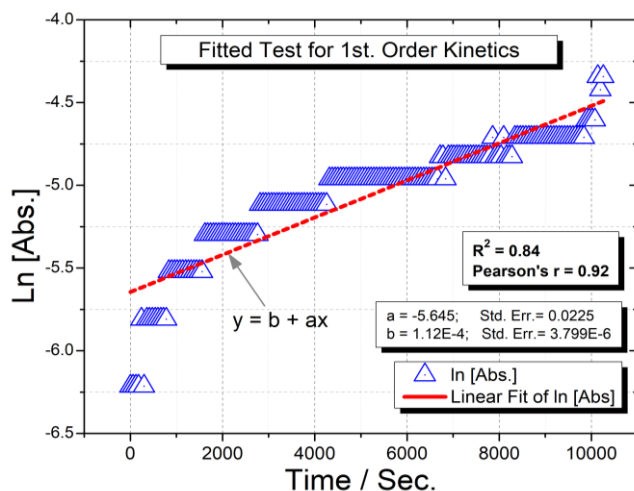
Figure 8(a): Fitted test for First - Order Kinetics
