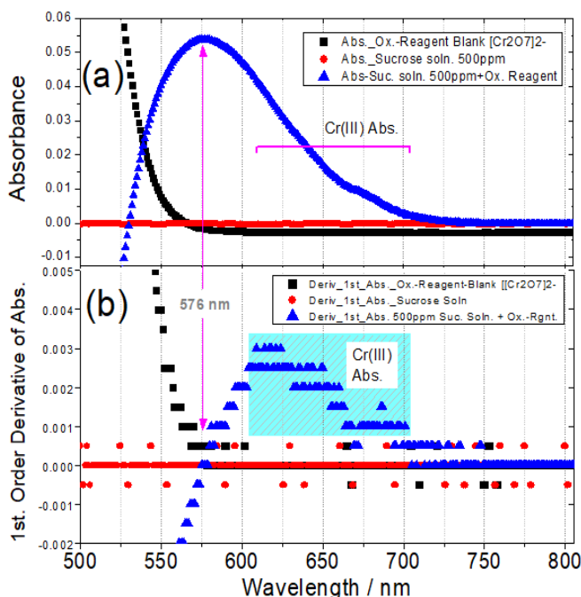
Figure 3: (a) Absorbance vs. wavelength and (b) The first - order derivative graph
