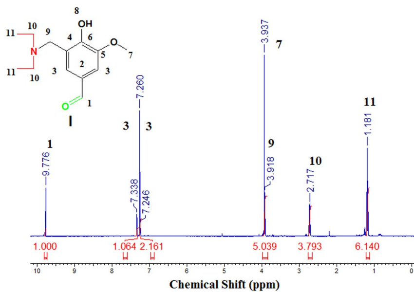
Figure 1: 1 H NMR (CDCl 3 ) of 2-[(diethylamino)methyl]-4-formyl-6-methoxyphenyl acrylate.
