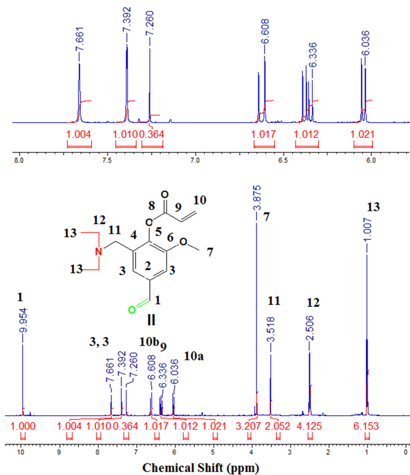
Figure 2: ^1\text{H} NMR ( \text{CDCl}_3 ) of 2-[(diethylamino)methyl]-4-formyl-6-methoxyphenyl acrylate (DEMAVA).
