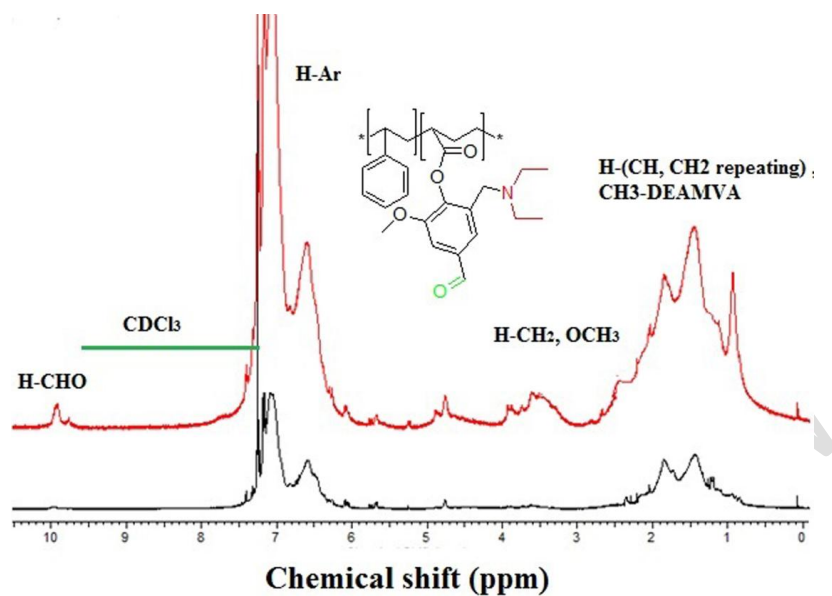
Figure 3: ^1\text{H} NMR spectra ( \text{CDCl}_3 ) of P(S- co -DEAMVA) 10, 25 mole ratio of DEAMVA
