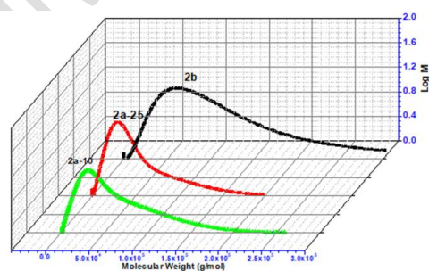
Figure 6: GPC molecular weight of copolymers
