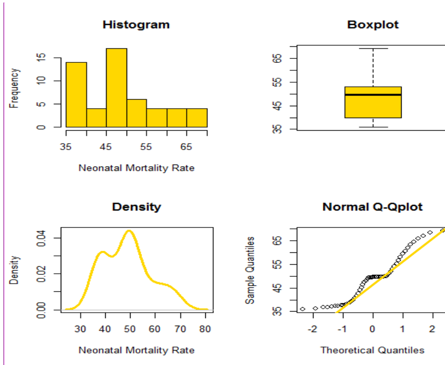
Figure 3: A graphical summary of the dataset
