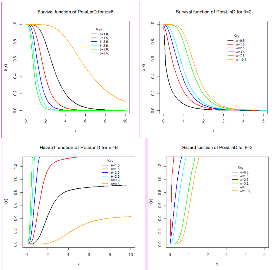
Figure 2: SF and HF of PoisLinD for Selected Values of the Parameters.
