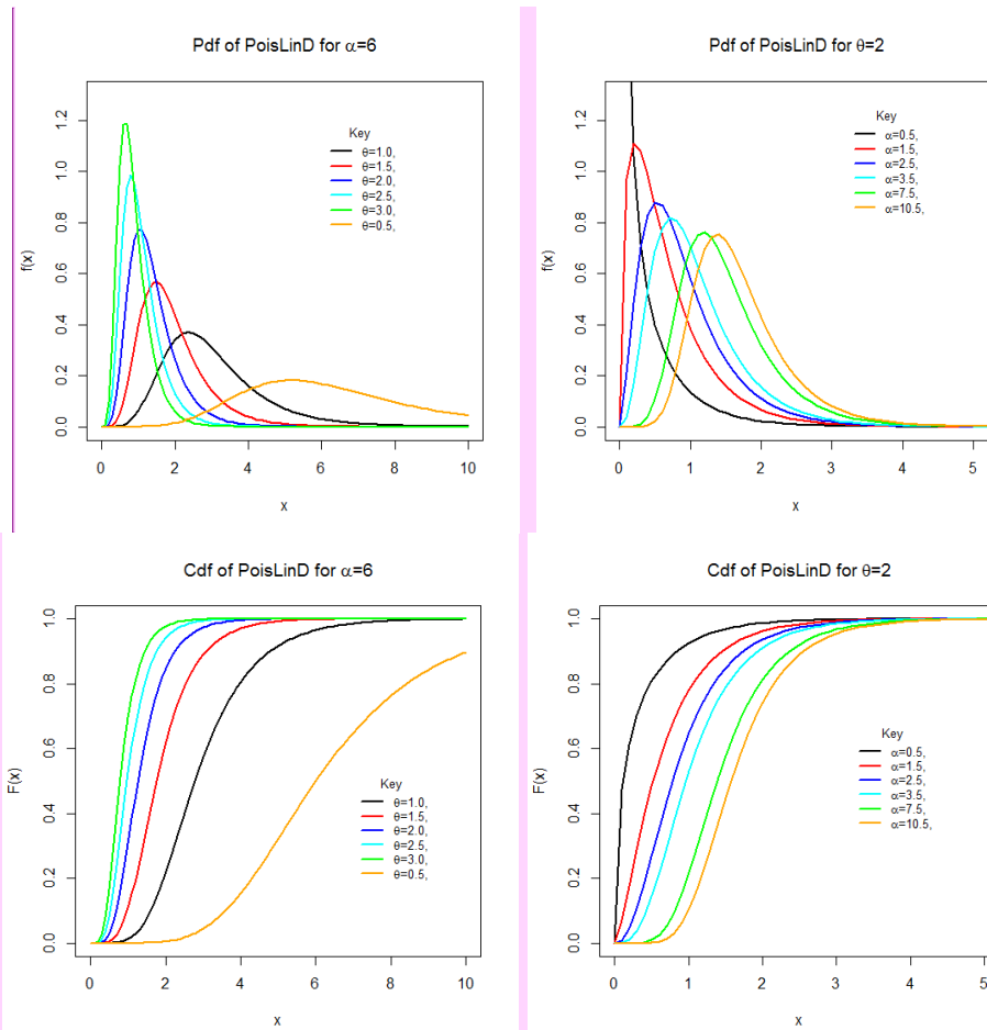
Fig. 1: PDF and CDF of the PoisLinD for different values of the parameters.
