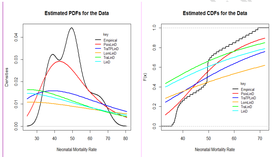
Figure 6: Estimated densities and cdfs of the fitted distributions to the Neonatal mortality rate data.
