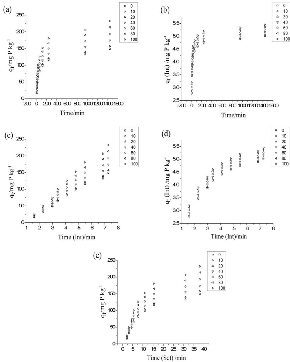
Fig1. The kinetics of P release by citric acid applied at 0, 10, 20, 40, 60, 80, 100 mM concentrations in highly calcareous soil having 17.5% free CaCO 3 as a function of time and similar data described by five kinetic models: Zero-order (a), First order (b), Simple elovich (c), Power (d) and parabolic functions (e)
