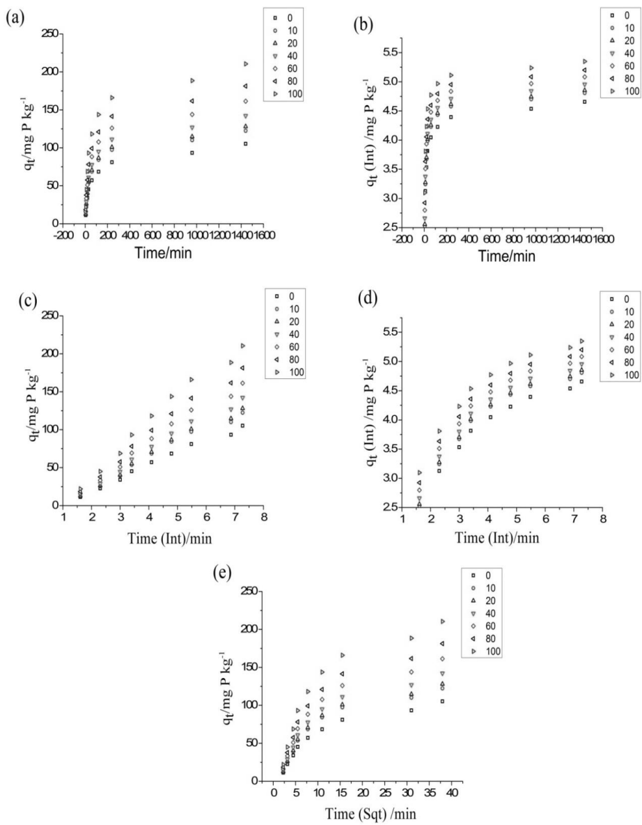
Fig. 2. The kinetics of P release by citric acid applied at 0, 10, 20, 40, 60, 80, 100 mM concentrations in highly calcareous soil having 21.5% free CaCO 3 as a function of time and similar data described by five kinetic models: Zero-order (a), First order (b), Simple elovich (c), Power (d) and parabolic functions (e)
