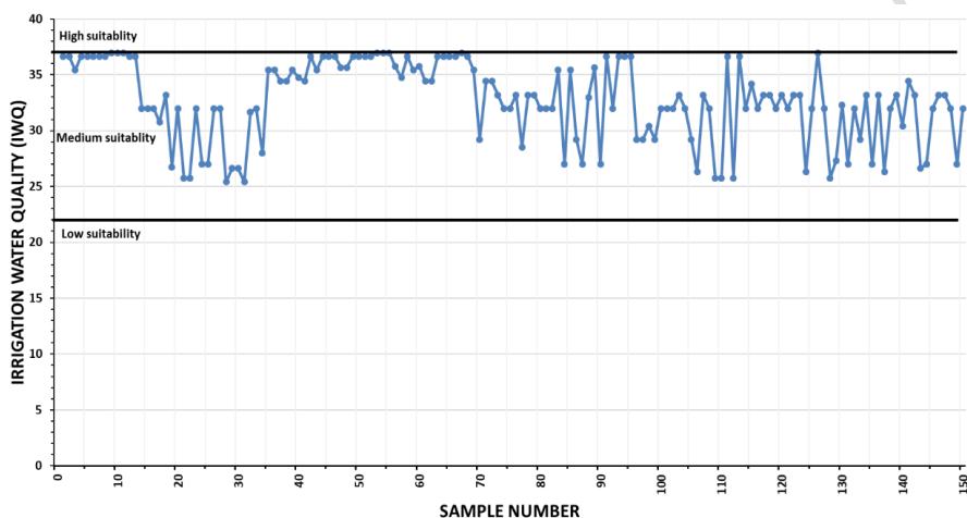
Fig. 8. Irrigation water quality index (IWQI) for 150 wells in Al-Jouf region, Saudi Arabia
