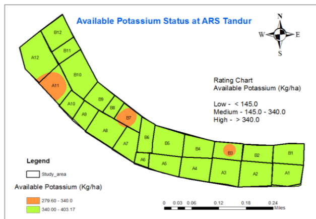
Fig. 6: Available soil \text{K}_2\text{O} ( \text{kg ha}^{-1} ) status of Research Station, Tandur.
