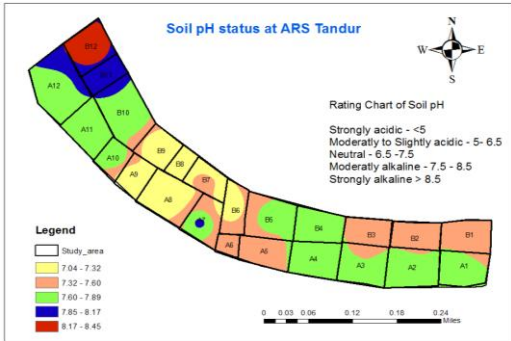
Fig 1: Soil pH of Agricultural Research Station, Tandur
