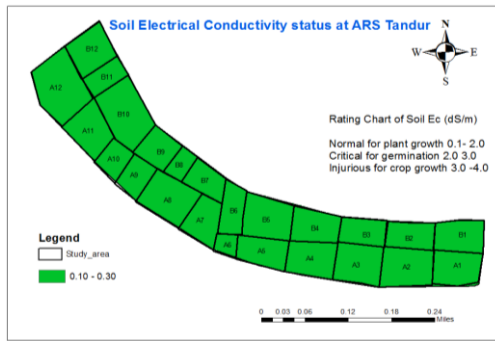
Fig 2: Soil EC of Agricultural Research Station, Tandur
