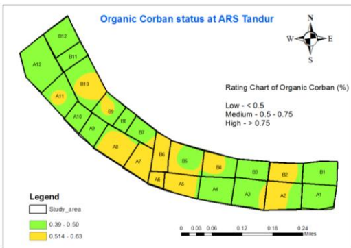
Fig 3: Soil OC (%) of Agricultural Research Station, Tandur
