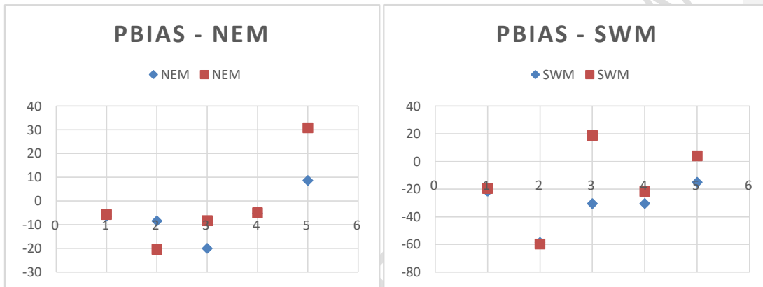
Fig.2.PBIASfor WSM-3 and Kessler Scheme during NEM 2021
