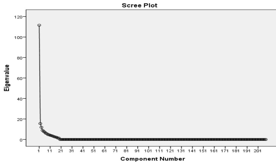
Fig 2. Scree plot obtained from PCA in SPSS
