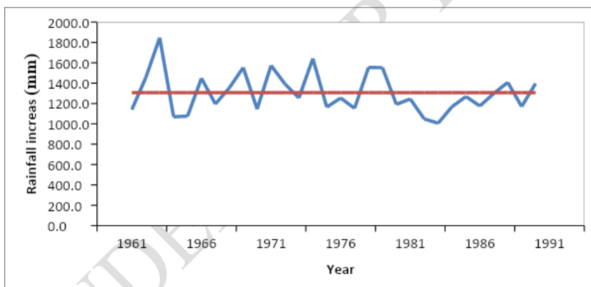
Figure 2: Year-to-year change in rainfall over the Kozah watershed from 1961 to 1990
