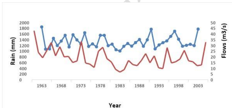
Figure 6: year to year change change in rainfall compared to flows of the Kara River from 1963 to 2003.
