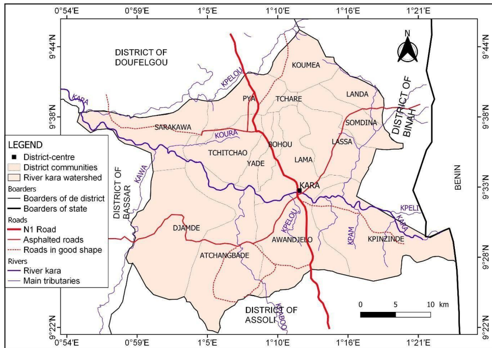
Figure 1: Geographical location of the Kara watershed.
