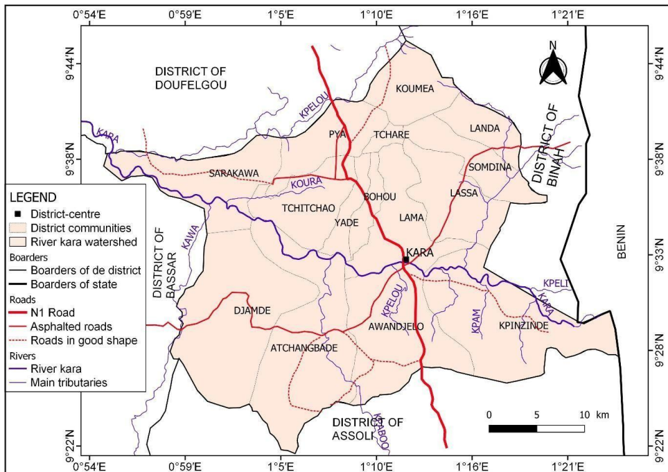
Figure 1: Geographical location of the Kara watershed in Kozah district.
