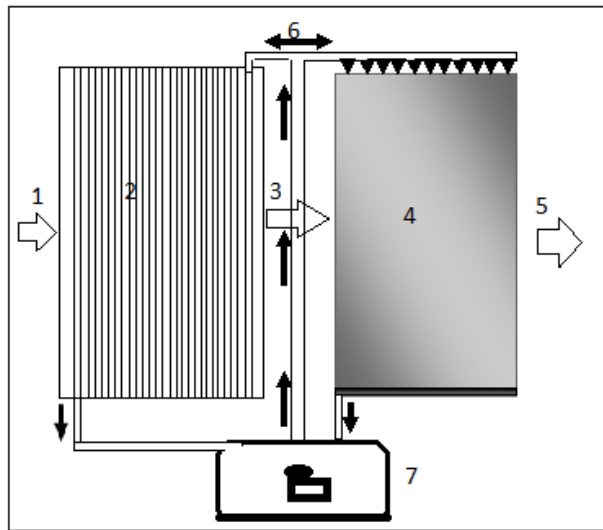
FIG1: SCHEMATIC ARRANGEMENT OF TSEC SYSTEM
