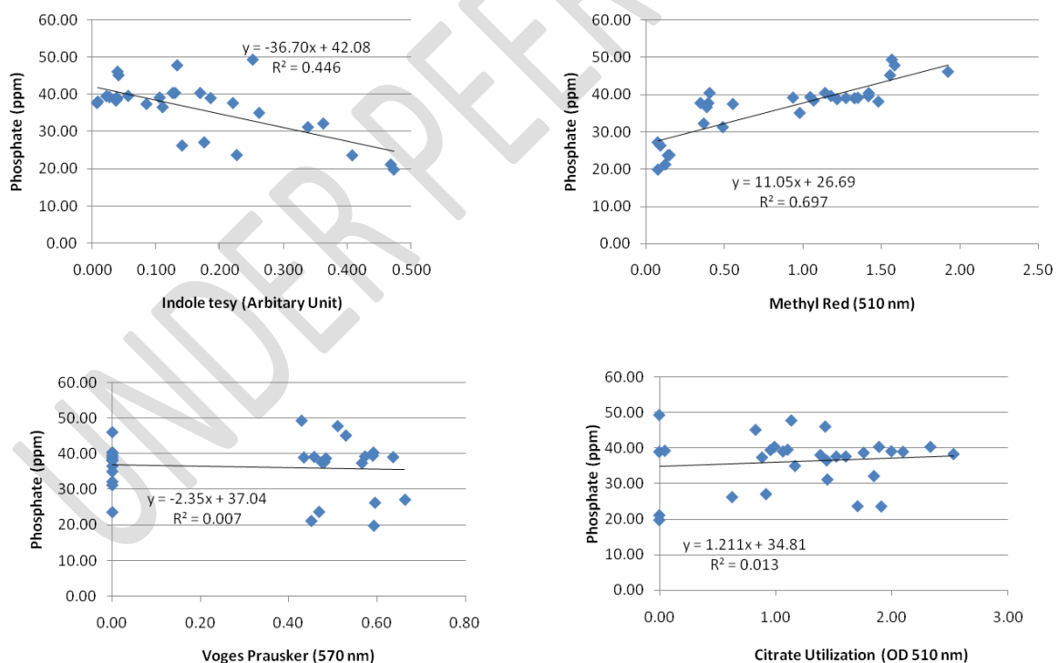
Figure 1: Correlation between IMViC parameters and P-solubilization activity. Correlation between P-solubilization and Indole test (Top left), methyl red test (top right), VoguesPrausker test (Bottom left) and citrate utilization test (bottom right).
