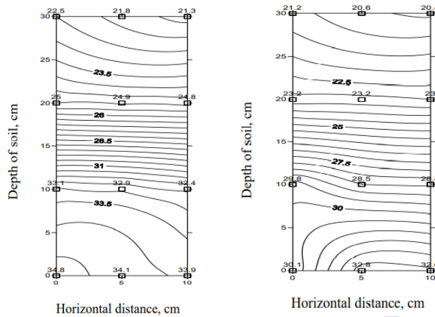
Fig. 4: Moisture distribution under plastic mulch & dried leaves next day after irrigation at 1.0 Epan
