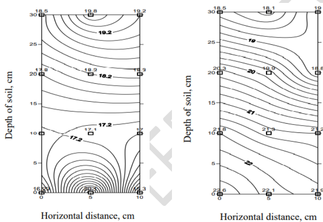
Fig. 9: Moisture distribution under no mulch day & paddy straw mulch day of irrigation at 0.6 Epan
