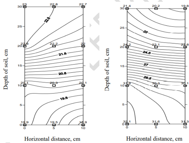
Fig. 3: Moisture distribution under no mulch & paddy straw mulch next day after irrigation at 1.0 Epan
