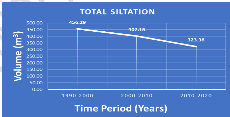
Fig 12: The total sedimentation in Brahmani Reservoir (1990-2000, 2000-2010 & 2010-2020)
