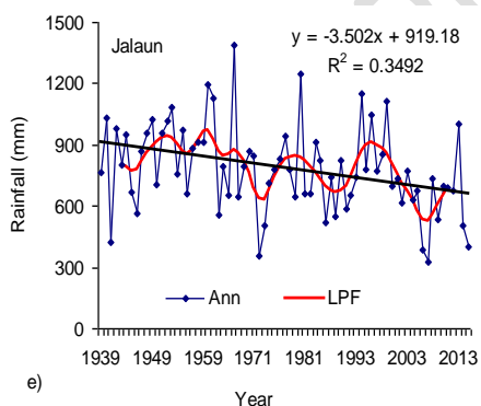
Fig 2 Mean annual (Ann) rainfall along with low pass filter (LPF) curve at different locations of Bundelkhand region of central India.
