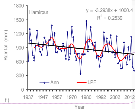
Fig 2 Mean annual (Ann) rainfall along with low pass filter (LPF) curve at different locations of Bundelkhand region of central India.
