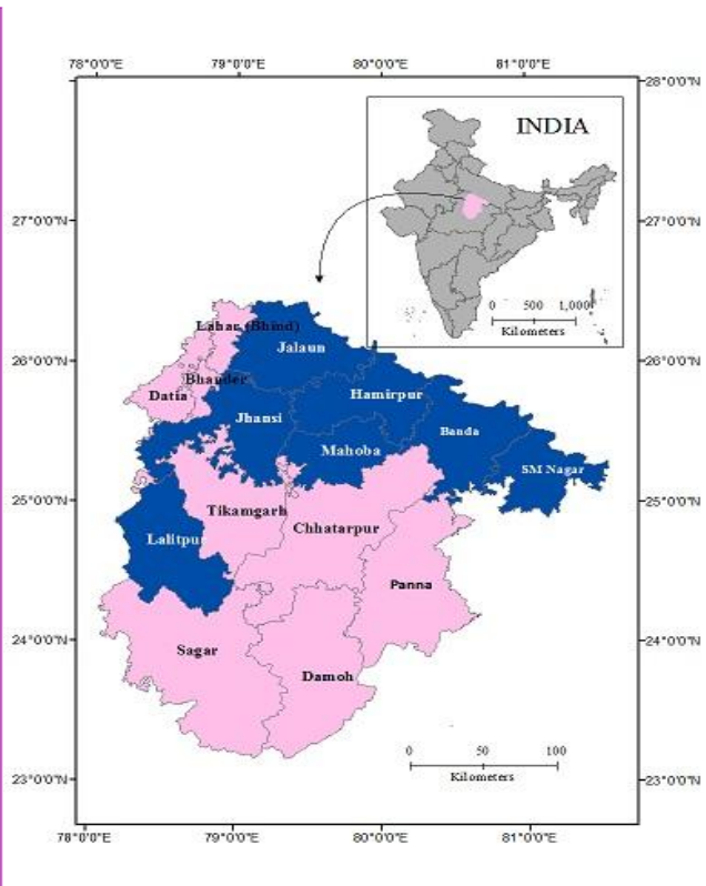
Fig 1 Location map of Bundelkhand region of central India.
