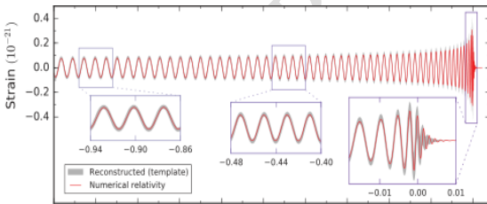
Fig.7 The original graph of gravitational waves of GW151226 calculated by using numerical relativity.
