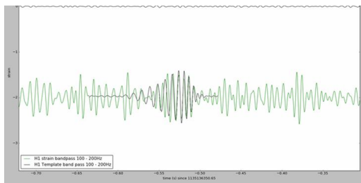
Fig.3 About 0.50 seconds before LIGO's so-called gravitational wave burst , the noise waveform (green curve) appeared in Hanford interferometer and the theoretical waveform calculated by numerical relativity (black curve).
