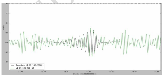
Fig.3 About 1.3 seconds before LIGO's
