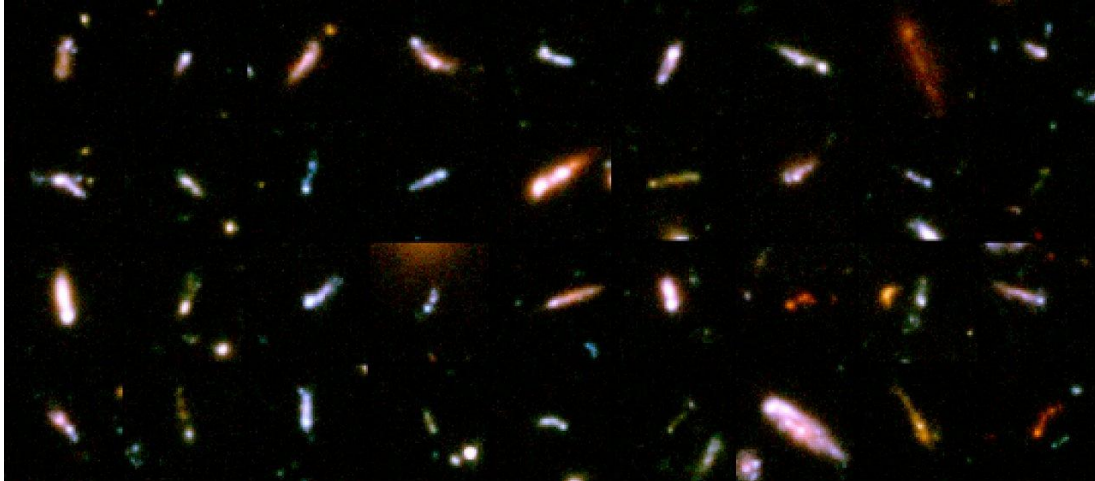
Fig. 9. A gallery of 36 Tadpole galaxies.
