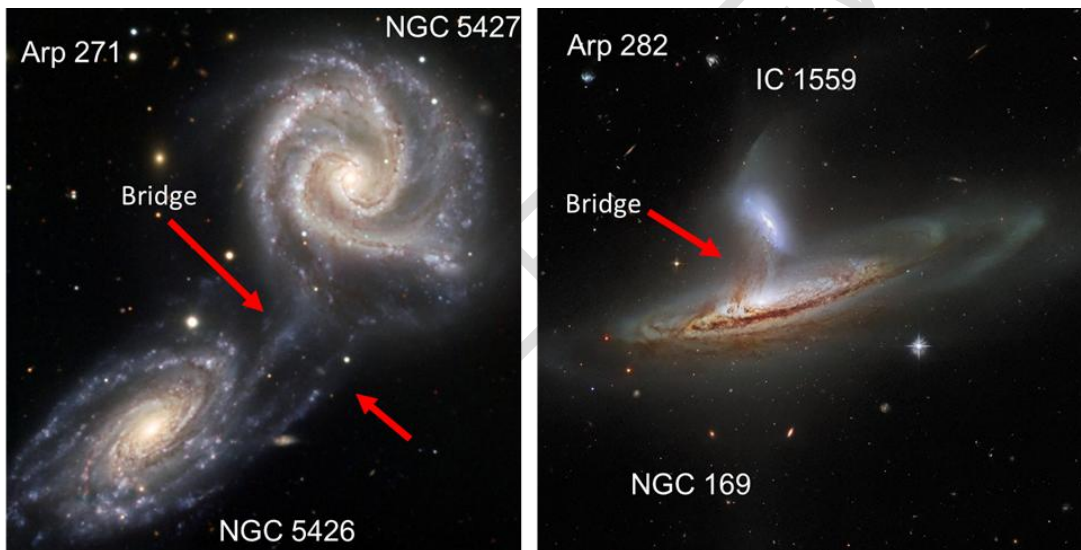
Fig. 2. Left is Arp 271, a pair of colliding galaxies NGC 5426 and NGC 5427 ; right is Arp282, a pair of colliding galaxies NGC 169 and IC 1559.
