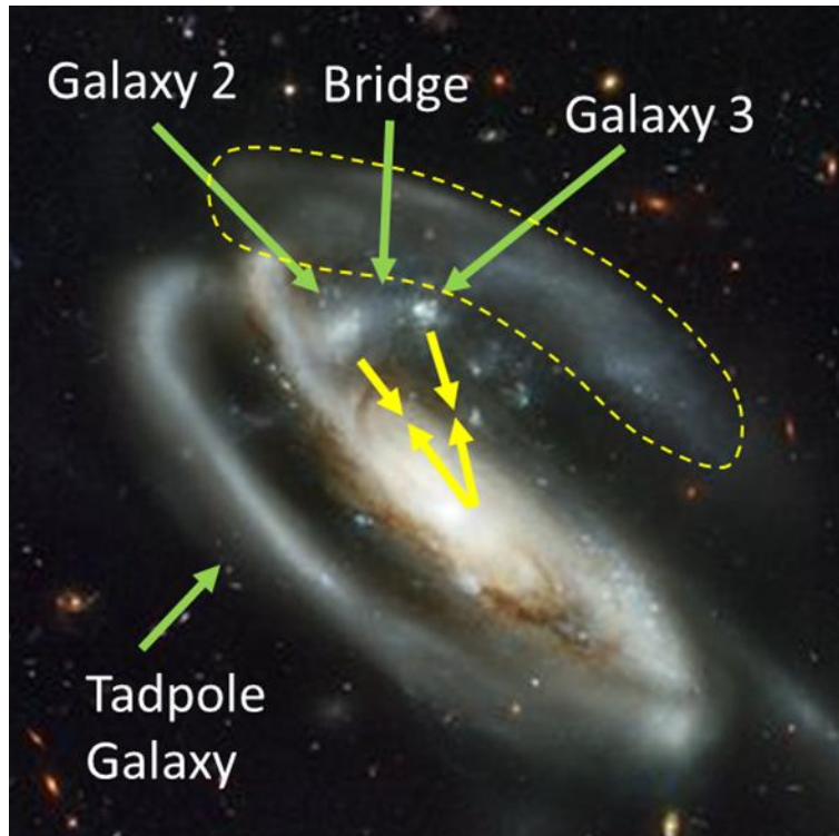
Fig. 5. Zoom-in image of Tadpole galaxy head
