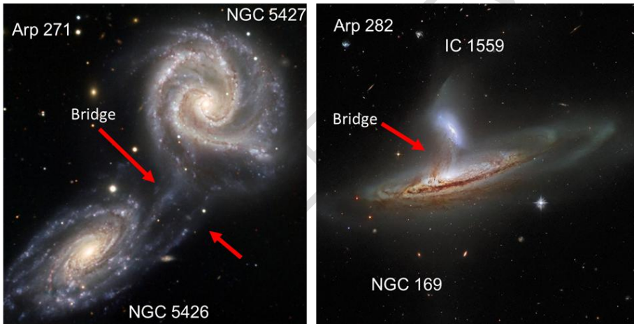
Fig. 2. Left is Arp 271, a pair of colliding galaxies NGC 5426 and NGC 5427 ; right is Arp282, a pair of colliding galaxies NGC 169 and IC 1559.
