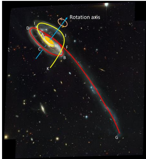
Fig. 4. Depicted spiral pattern of the Tadpole galaxy
