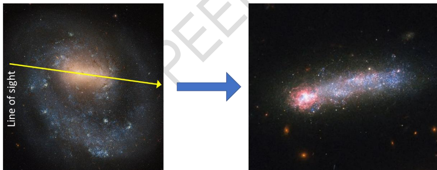
Fig. 10. Illustration of converting a one-arm galaxy to a Tadpole galaxy with edge-on and line of sight parallel to the galactic bar. Left is the one-arm galaxy NGC 4618, right is the galaxy LEDA 36252. Please note, the LEDA 36252 may not be the case.
