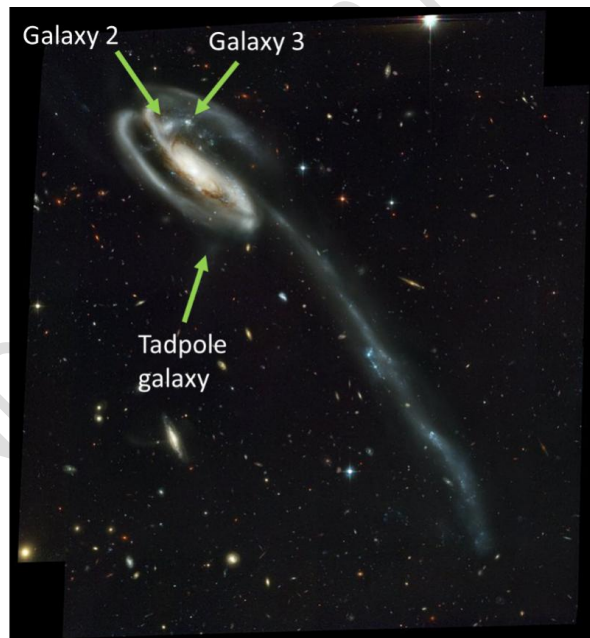
Fig. 1. The image of the Tadpole galaxy UGC 10214 with labeled 3 galaxies as a local galactic cluster. The image is credited to: NASA, H. Ford (JHU), G. Illingworth (UCSC/LO), M. Ciampin (STScI), G. Hartig (STScI), the ACS Science Team, and ESA.
