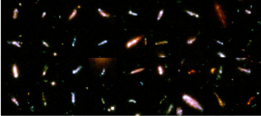
Fig. 9. A gallery of 36 Tadpole galaxies.
