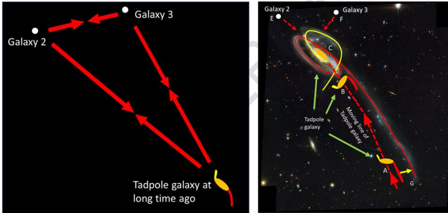
Fig. 7. Left is the illustration of the cluster of the Tadpole galaxy and two smaller galaxies at long time ago; right is the proposed moving lines of the three galaxies.
