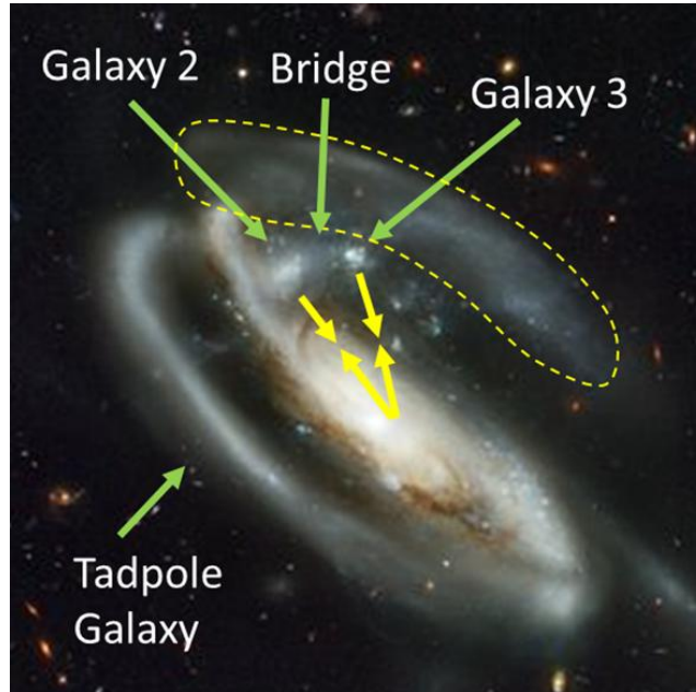
Fig. 5. Zoom-in image of Tadpole galaxy head
