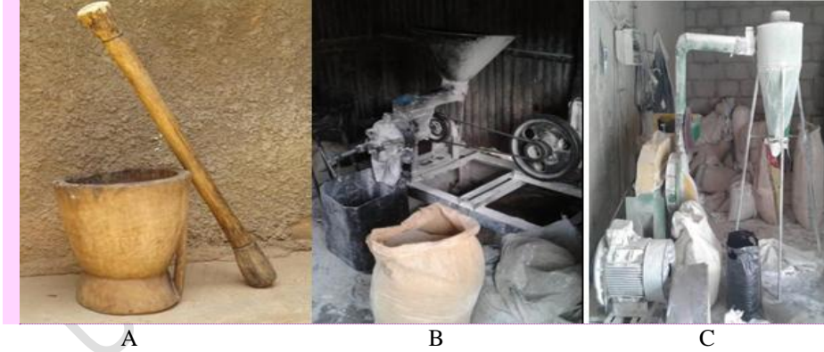
Figure 2: Grinding methods: (A) mortar and pestle; (B) Hammer mill and (C) Disc Mill.
