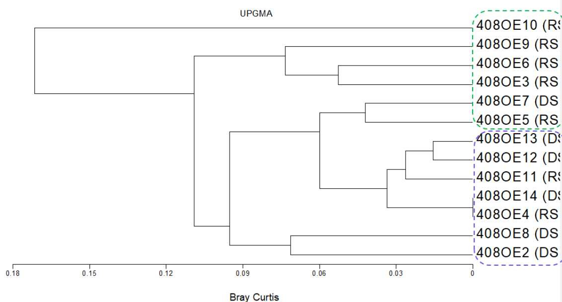
Figure 2. Results of cluster analysis considering 18 terpenes that concomitantly occur in the 13 essential oils obtained from the leaves of Osteophloeum platyspermum (Myristicaceae). Blue dots = dry season; green dots = rainy season.
