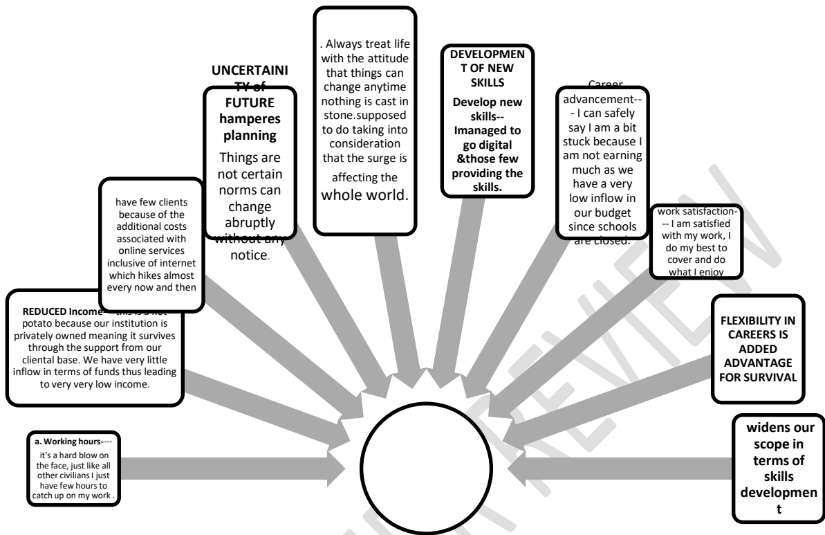
Figure 1. Clusters
