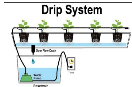
Fig.5 Drip System
