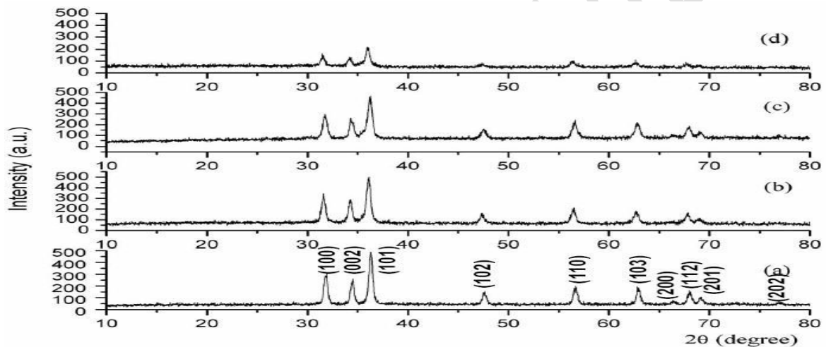
Fig-1 XRD method in samples are annealed in ambient air at 500° to 550° 1 hours 30 mins.. (a) undoped ZnO; (b) 1mol% Mn doped ZnO; (c) 2 mol% Mn doped ZnO and (d) 3 mol% Mn doped ZnO.
