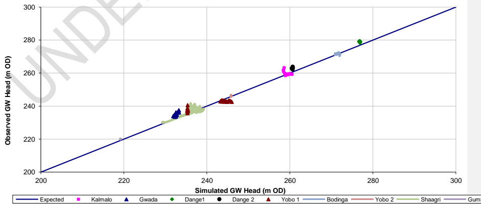
Fig. 4a. Observed and Simulated Groundwater Heads for all Observation Boreholes
