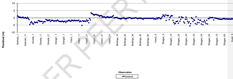
Fig.4c. Residual Analysis Plot for the Observed and Simulated GW Head
