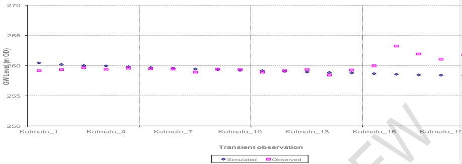
Fig 4b. Observed and Simulated GW Heads Obtained at Kalmalo BH (S33 09)
