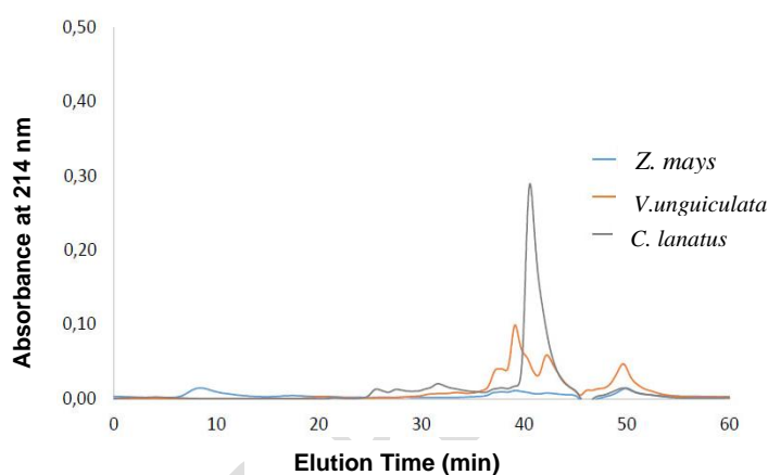
Figure 3. HPLC profiles of aqueous extracts 204-35000 Da
