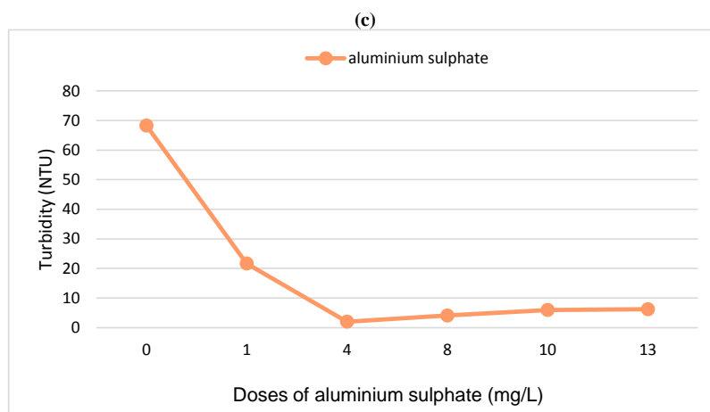
Figure 5: Turbidity variation of the raw water sample of 68.69 NTU as a function of coagulant solution doses
