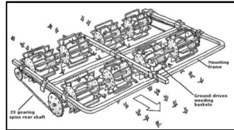
Fig. 1: Basket weeder for inter-row weed control (Bowman 1997)
