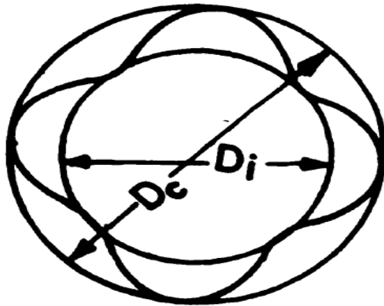
Fig.3 Diagram of smallest circumscribing and largest inscribing circles of a particle
