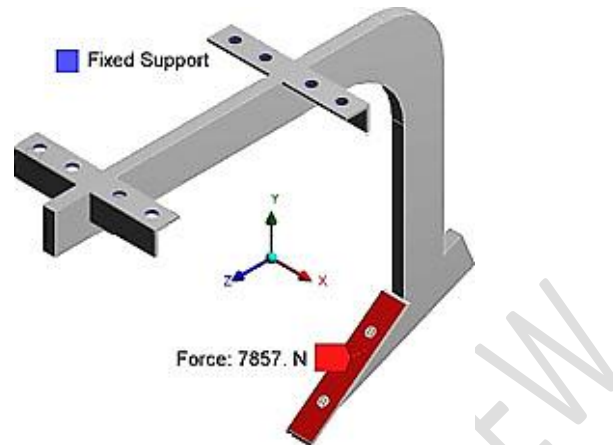
Fig. 2. Force and constraints on the straight subsoiler
