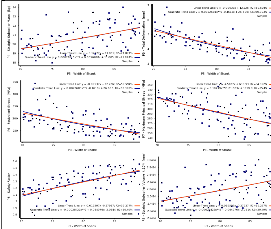
Fig. 7. Linear and quadratic relationships between P3 and the output variables
