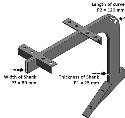
Fig. 1. Design parameters of Inclined subsoiler
