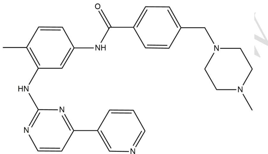
Fig.1 The structure of Imatinib
