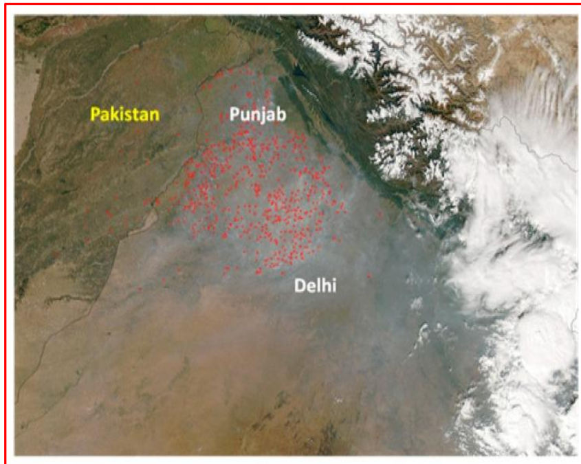
Figure - 3 Crop Burning captured by NASA
