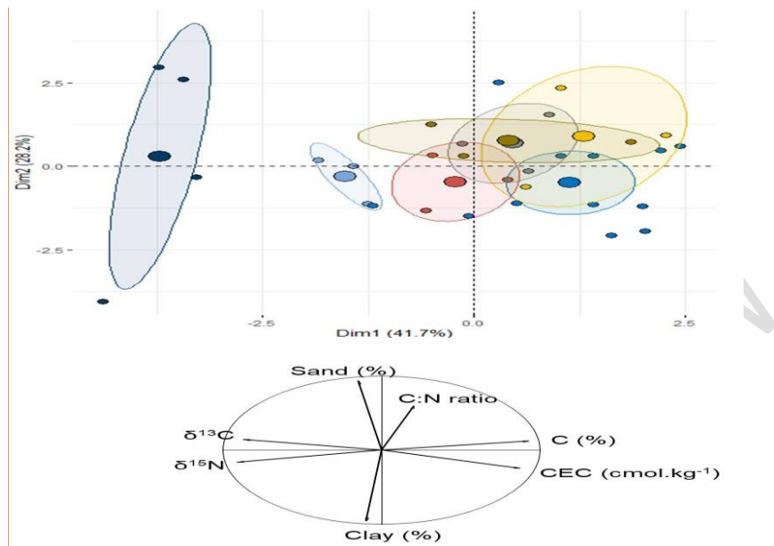
Fig. 1. Principal component analysis (PCA) and correlation circle of the soil physical and chemical properties of termite mound soils, CAT nest , CAT periph , LENT small , LENT medium and LENT large and the control soil sampled at 0-5cm depth or at 50-100 cm depth. The arrow and the circle represent the different trajectories between CAT, LENT and CTRL.
