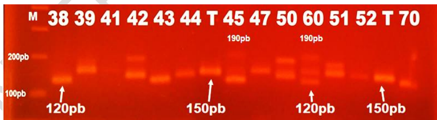
Figure 5: Electrophoresis gel showing individuals having three bands
