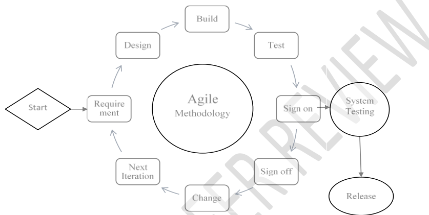
Figure 1: Agile Model
