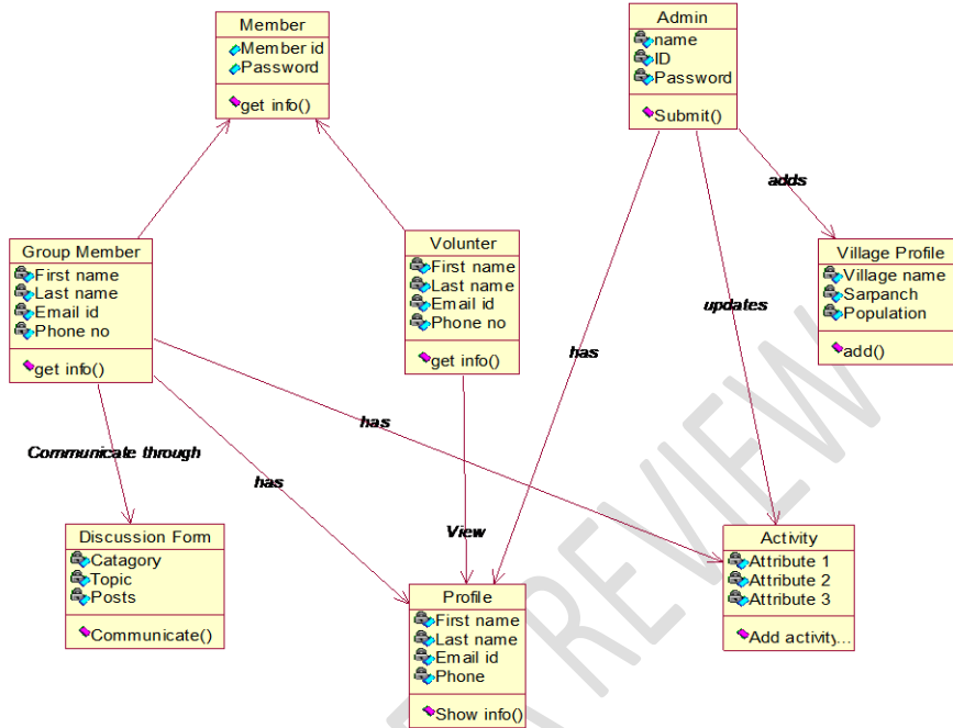
Figure 7: Class Diagram
