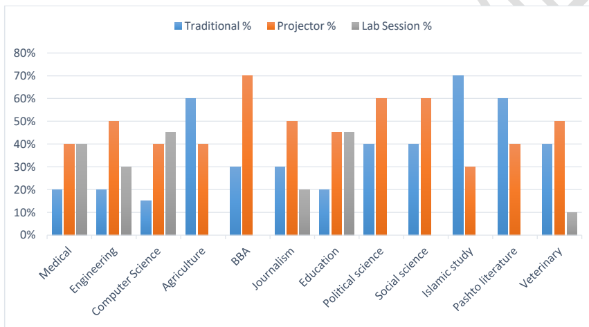
Fig. 3: Contents delivery
