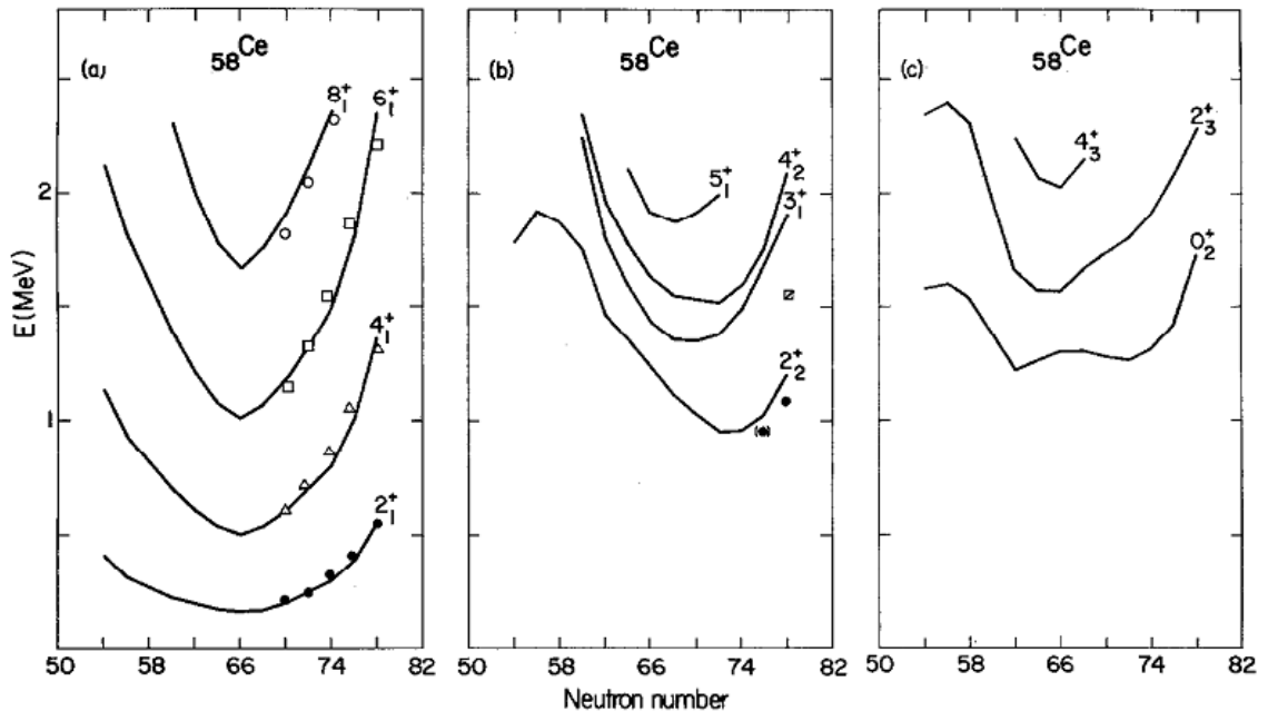
Figure (1): Comparison between calculated and experimental energy levels in Ce. The experimental levels are taken from refs. [11-18].( specify which is experimental , and which is theoretical on this Fig. )
