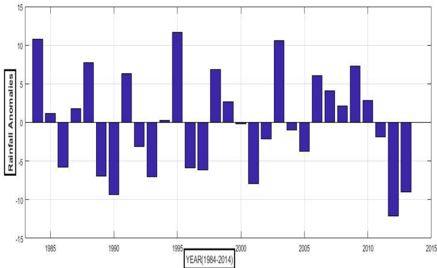
Figure 3 : Rainfall Anomalies from 1984-2013
