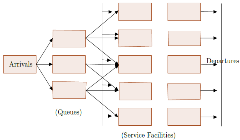
Figure 5: Multiple servers, Multiple-phases System
