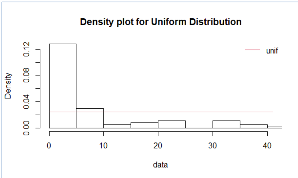
Fig 3.3: Uniform Distribution Probability Density Curve of Weekly Number of Confirmed Cases of Lassa fever in Edo State
