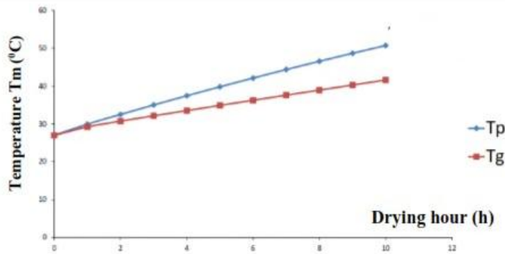
Fig .7. Temperature profile of the small dryer (Tp) and the large dryer (Tg) after 10 h of functioning
