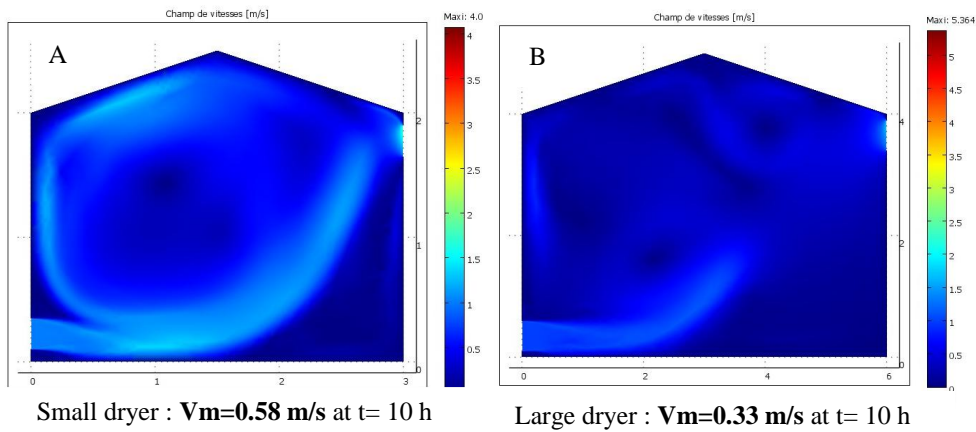
Fig .8. Internal velocity fields in the small (A) and the large (B) dryer
