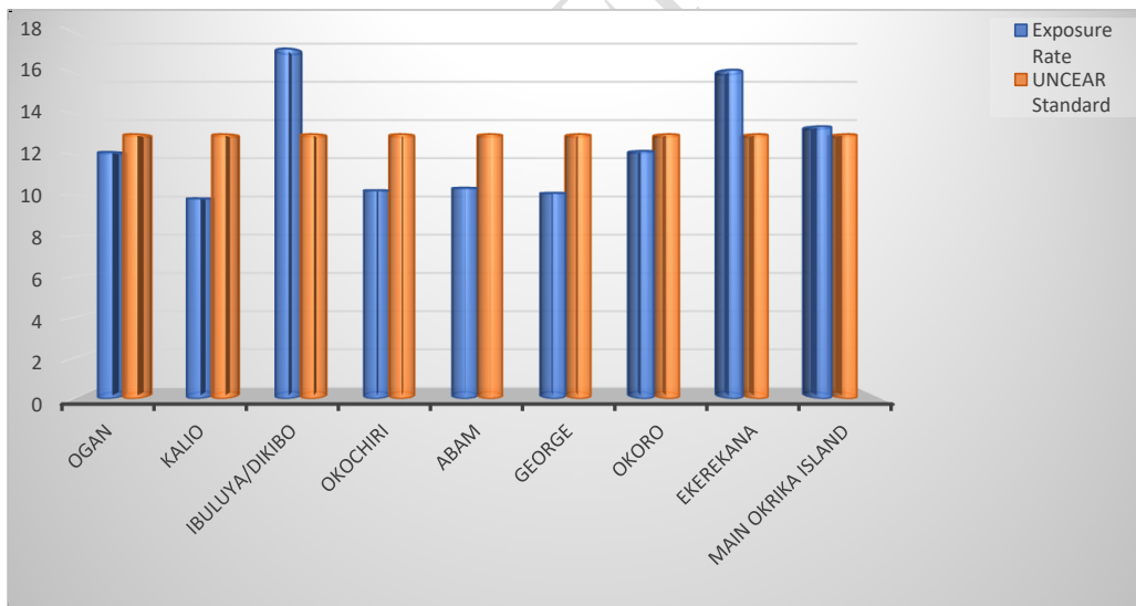
Figure 8. Comparison of exposure rate with UNSEAR, 2000
