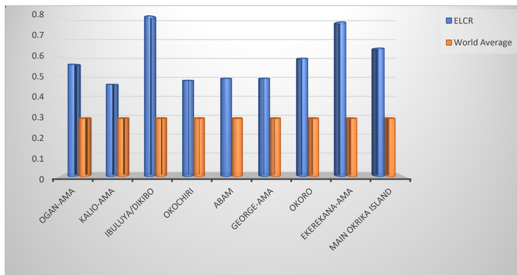
Figure 11. Comparison of ELCR with world average. UNSCEAR, 2000
