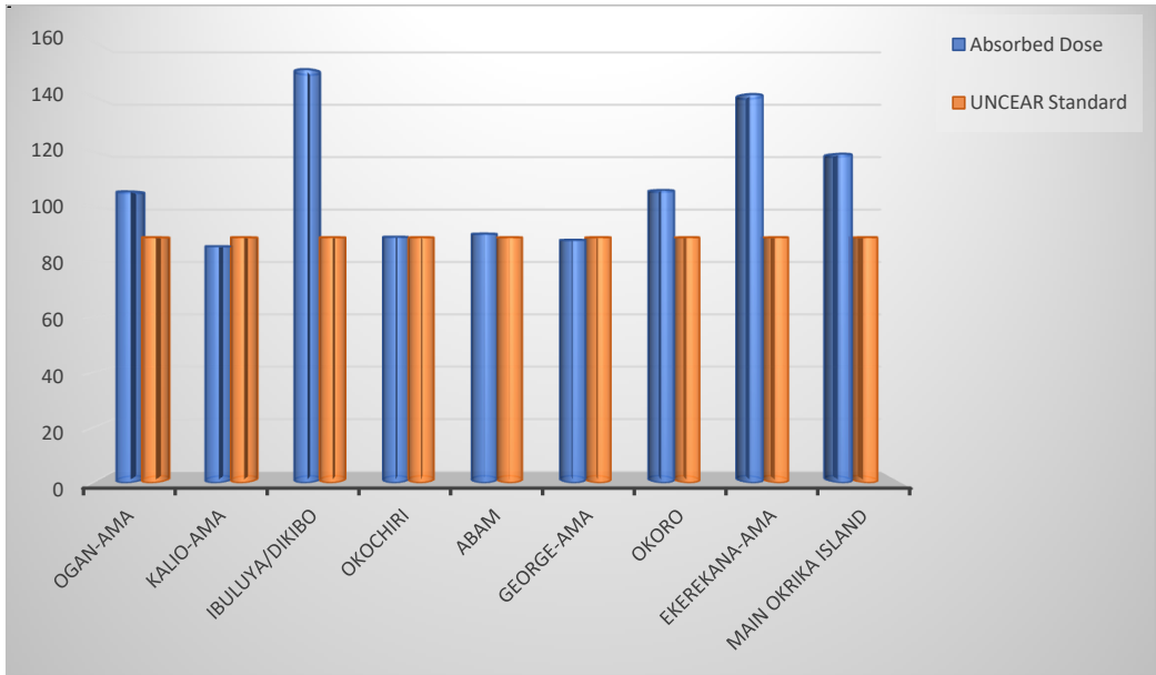
Figure 9. Comparison of absorbed dose rate with UNSCEAR, 2000
