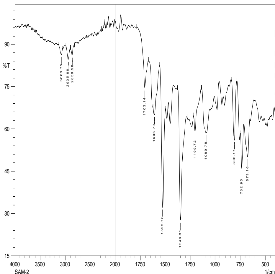
Fig. 3 FTIR of MNB
