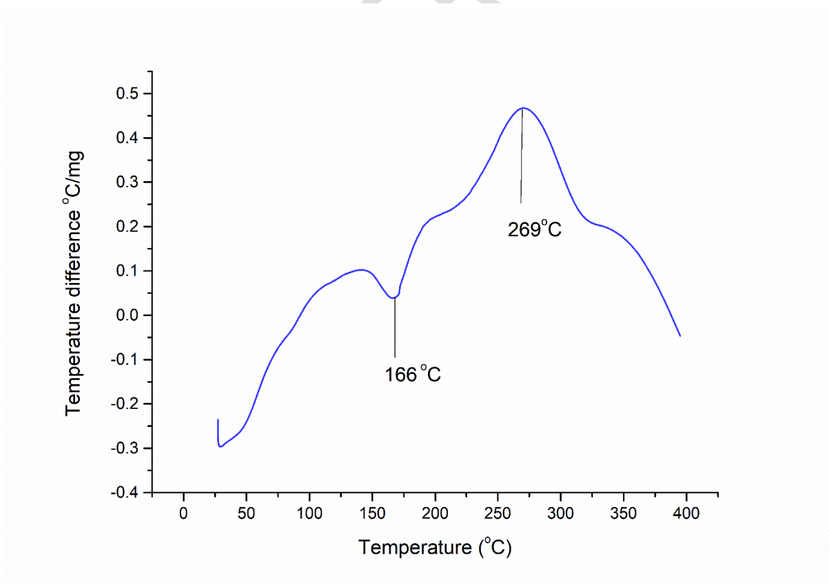
Fig.6 DTA curve of MNB
