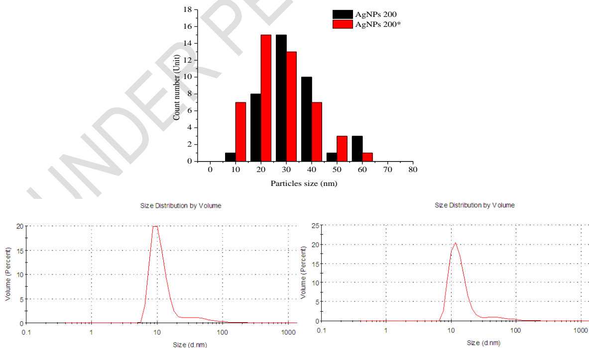
Fig. 6 Particle size distribution (a) size distribution by volume of AgNPs 200* (b) AgNPs 200 (c)
