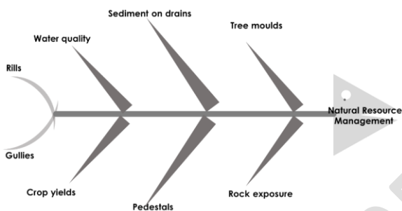
Figure 1: An illustration on the association between soil erosion monitoring indicators and natural resource management
