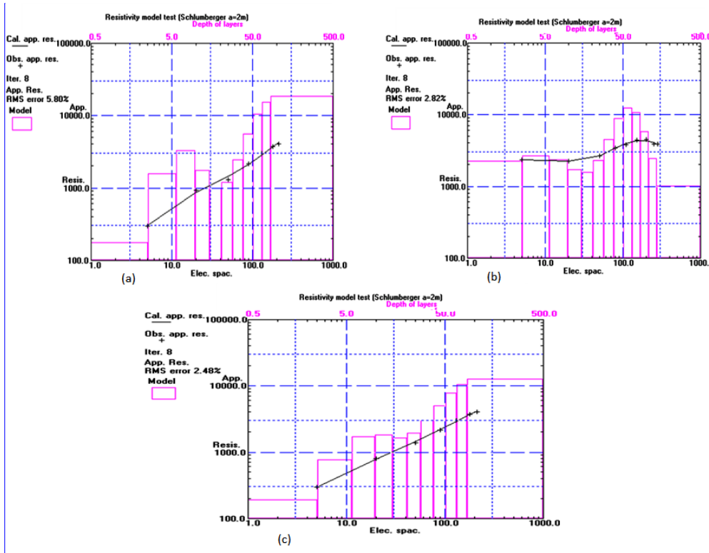
Fig. 6: (a) Inverted model layer for VES 5 taken at Iguebe south (2) Inverted model layer for VES 6 taken at Ebelle (c) Inverted model layer for VES 7 taken at Ekpon in Edo State
