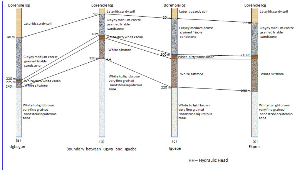
Fig.8:Litho-log of boreholes section of the study area(Source of borehole data: Rock Well Drilling Company)
