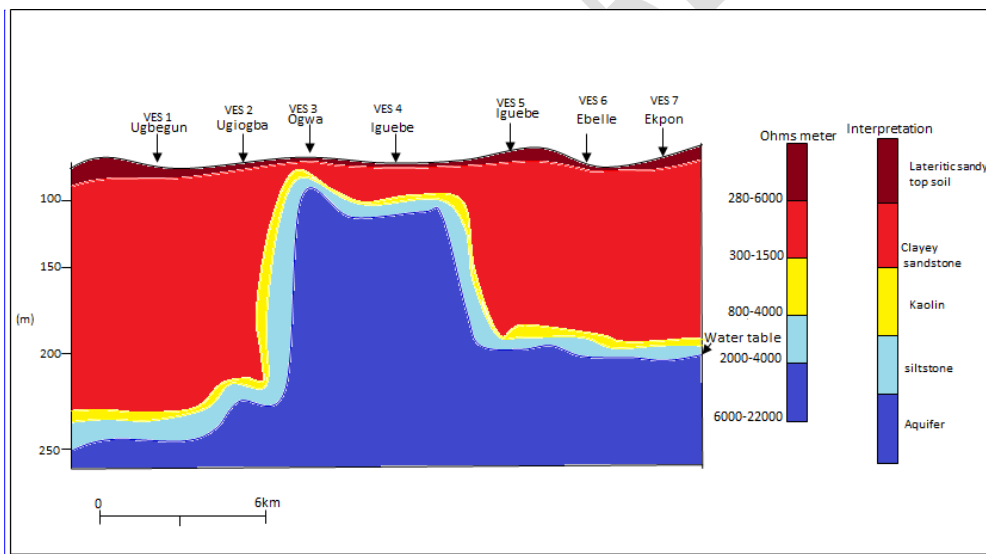
Fig. 7: Geo-electrical resistivity section of the study area
