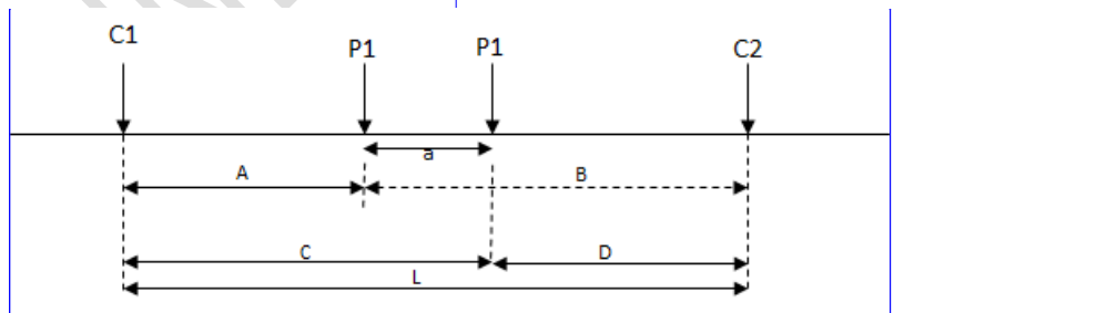
Fig. 4: Schlumberger array (After Lowrie, 1997)
