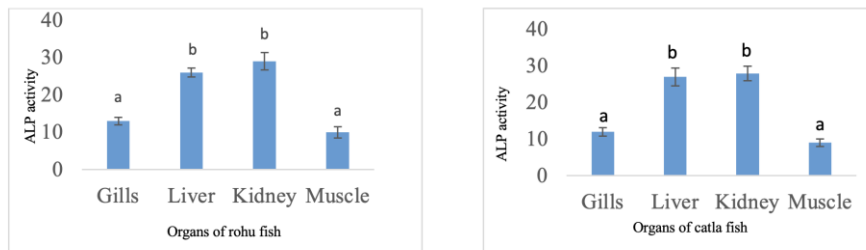
Fig. 6. ALP activity as n moles of para-nitrophenol \text{mg protein}^{-1} ( 37^\circ\text{C} ) in different organs of cultured Rohu fish and Catla fish. Bars with different letters (a and b) differ significantly ( P < 0.05 )
