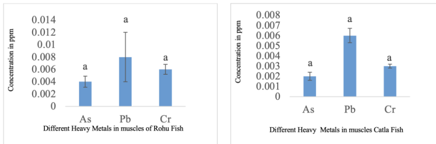
Fig. 4. Different heavy metals concentration in muscles of cultured rohu fish and catla fish. Bars with different letters (a and b) differ significantly ( P < 0.05 )
