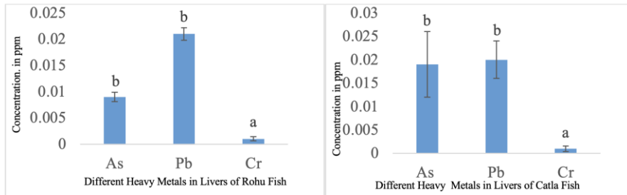
Fig. 2. Different heavy metals concentration in liver of cultured rohu fish and catla fish Bars with different letters (a and b) differ significantly ( P < 0.05 )
