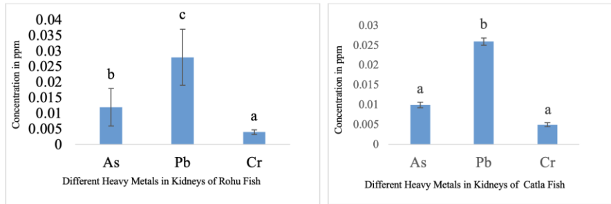
Fig. 3. Different heavy metals concentration in kidney of cultured rohu fish and catla fish. Bars with different letters (a and b) differ significantly ( P < 0.05 )
