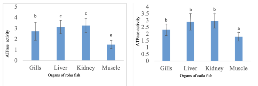
Fig. 5. ATPase activity as \mu\text{g} of phosphorus \text{mg protein}^{-1} per min ( 37^\circ\text{C} ) in different organs of cultured rohu fish and catla fish. Bars with different letters (a and b) differ significantly ( P < 0.05 )
