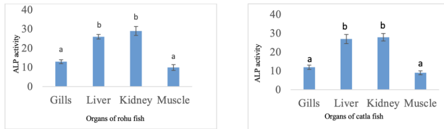
Fig. 6. ALP activity as n moles of para-nitrophenol mg protein-1 (37°C) in different organs of cultured Rohu fish and Catla fish. Bars with different letters (a and b) differ significantly (P<0.05)
