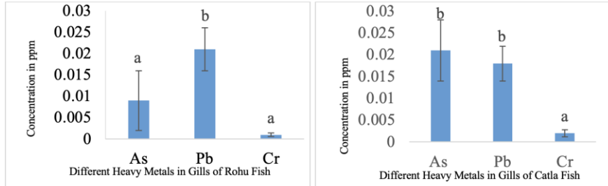
Fig. 1. Different heavy metals concentration in gills of cultured rohu fish and catla fish Bars with different letters (a and b) differ significantly ( P < 0.05 )
