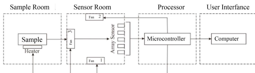
Figure 3. Electronic Nose System Block Diagram [19]
