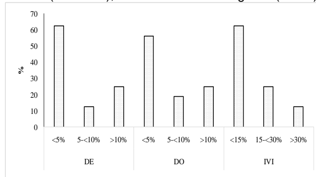
Figure 3. Class distribution of herbaceous grass species in the tropical savanna of West Timor (DE = Density, DO = dominance, and IVI = Importance Value Index)
